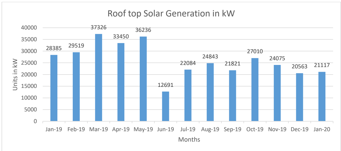
Fig 3: Monthly roof-top solar Energy Generation- 2019-20
